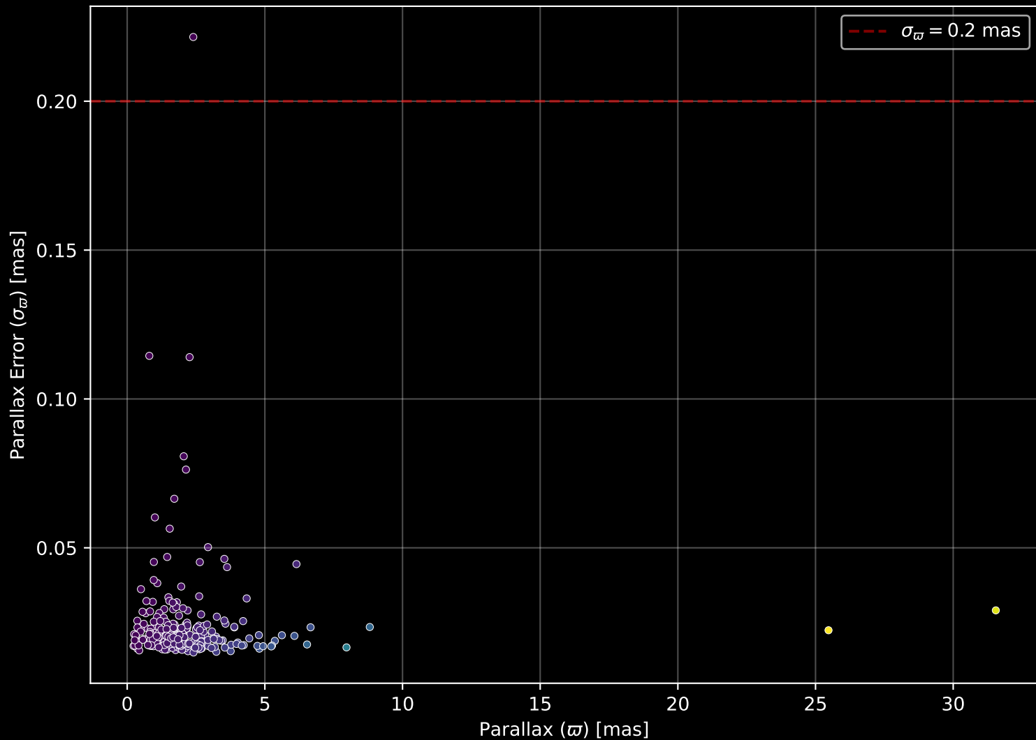
GALAH DR4 Field: [6882] Parallax Quality (n= 276)
