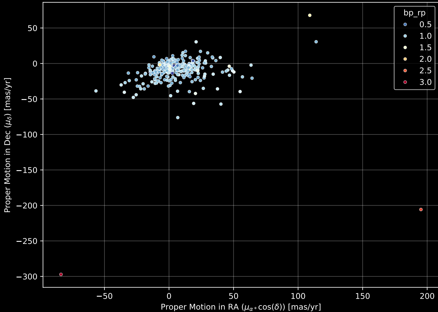
GALAH DR4 Field: [6882] Proper Motion Diagram (n= 276)
