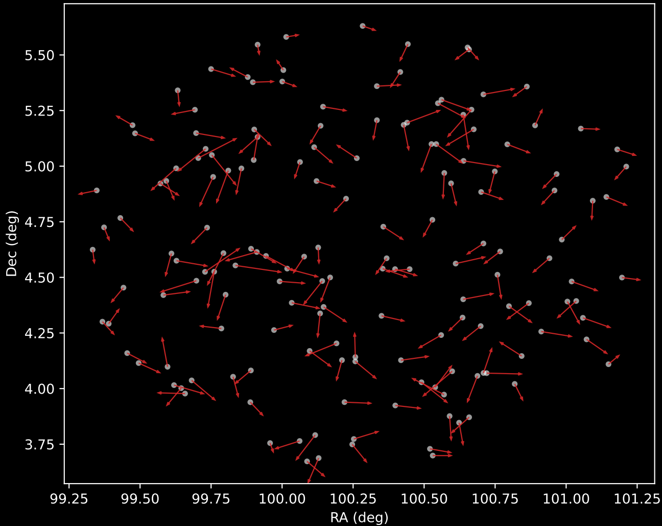
GALAH DR4 Cluster 6 Proper Motion Vectors (n=160)
