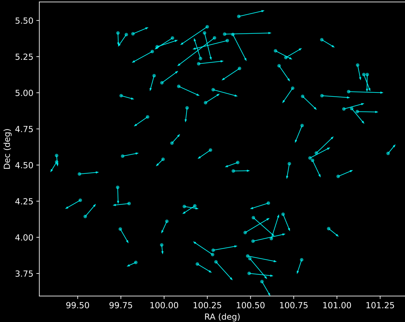
GALAH DR4 Noise Stream Proper Motion Vectors (n=80)
