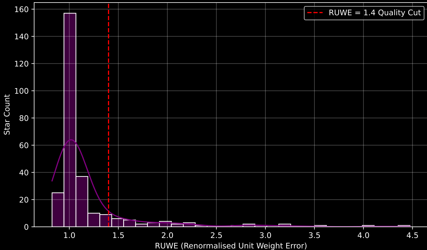
GALAH DR4 Field [6882] RUWE Distribution (n= 273)
