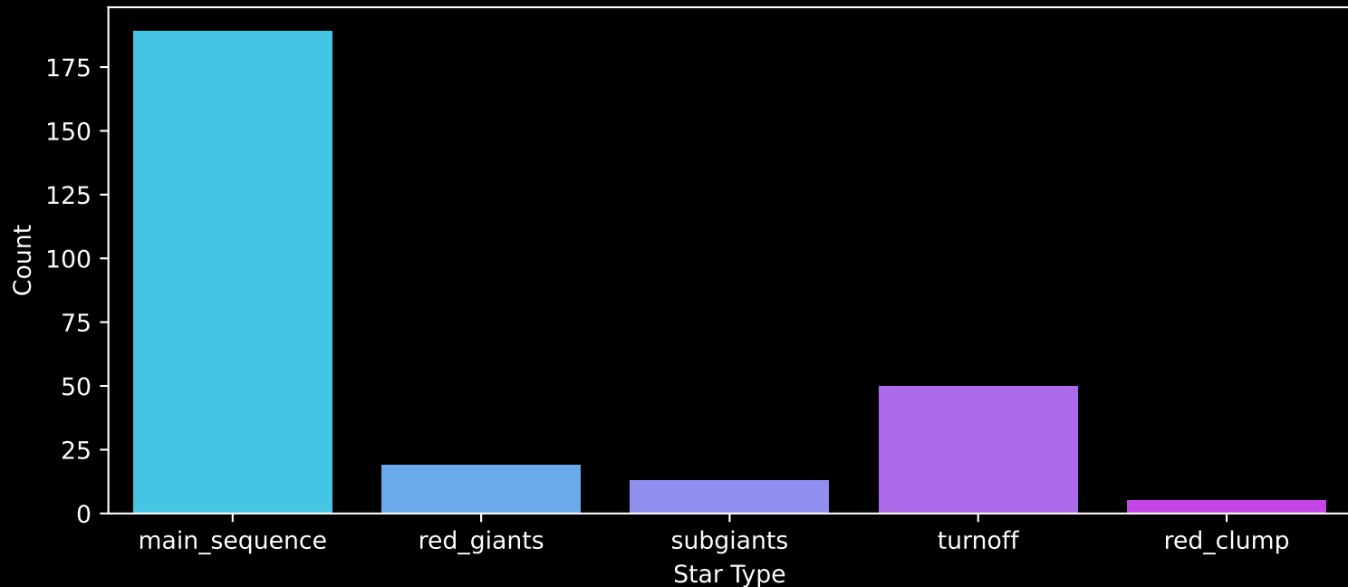
GALAH DR4 Field: [6882] Count plot of Star Type
