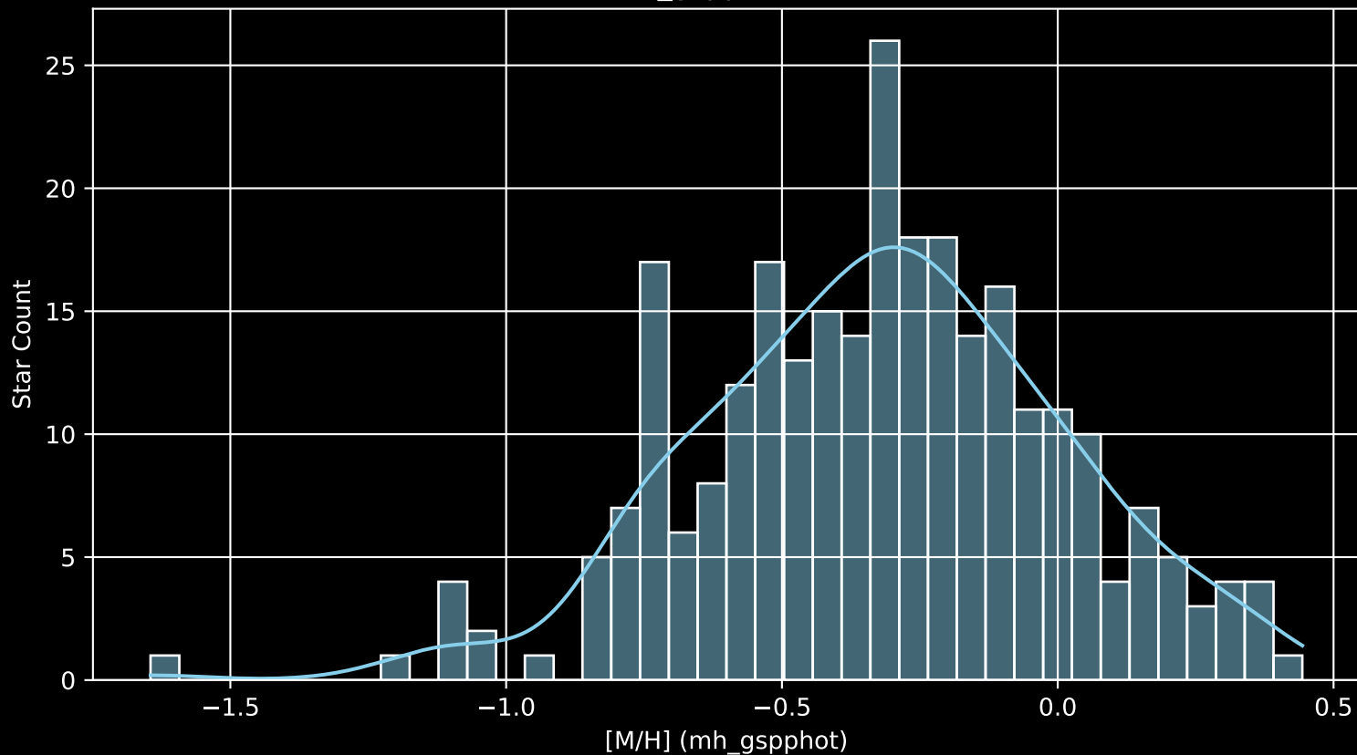
GALAH DR4 Field: [6882] [M/H] (mh_gspphot) (n= 275)
